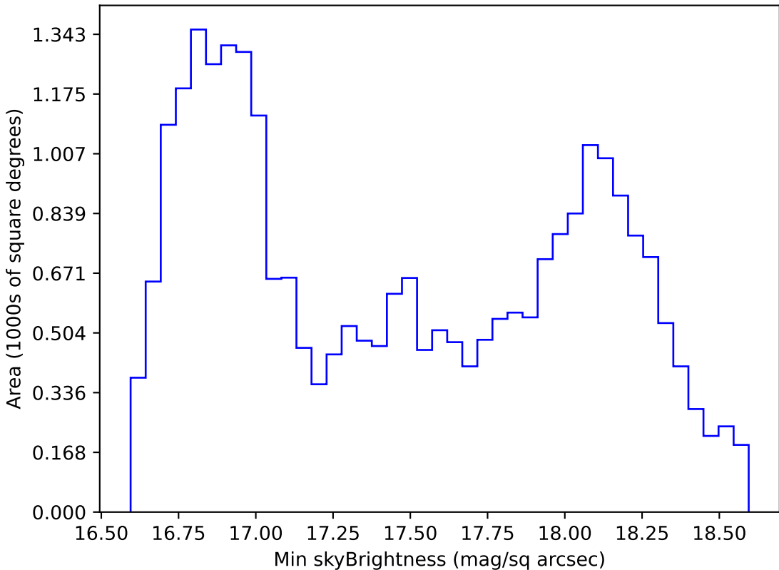
roll_pause_mjdp120_v3.4_10yrs All sky z band: Min skyBrightness
