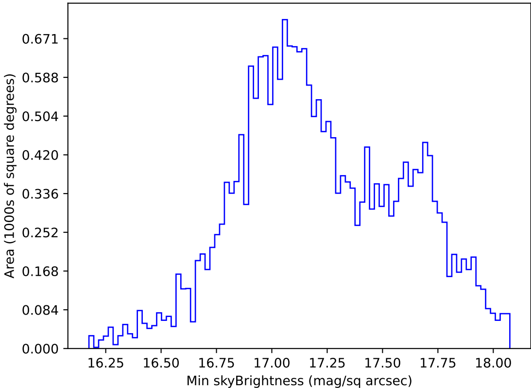
roll_pause_mjdp120_v3.4_10yrs All sky y band: Min skyBrightness
