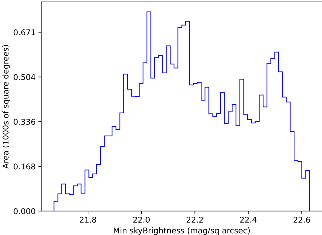
roll_pause_mjdp120_v3.4_10yrs All sky u band: Min skyBrightness
