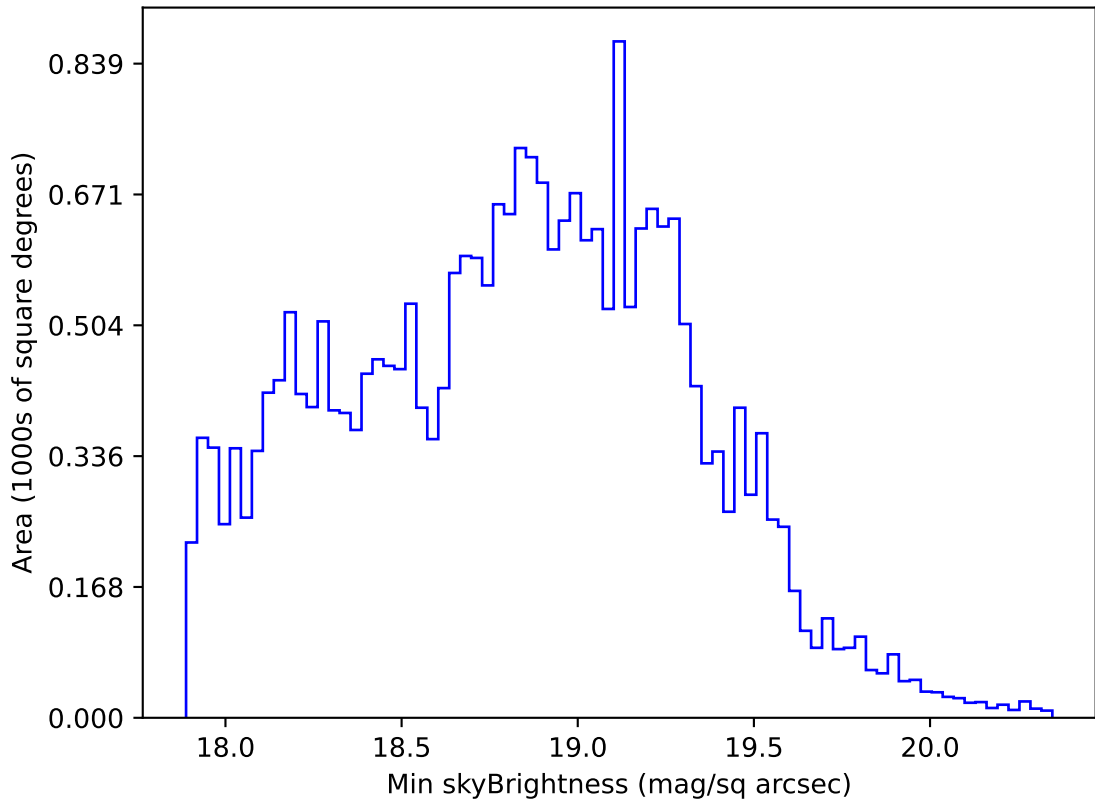
roll_pause_mjdp120_v3.4_10yrs All sky r band: Min skyBrightness
