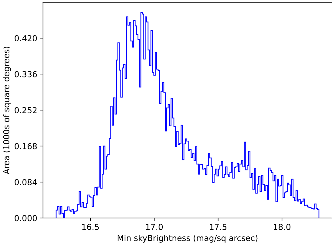
roll_pause_mjdp120_v3.4_10yrs All sky all bands: Min skyBrightness
