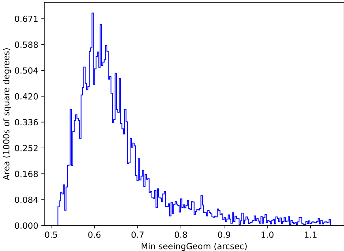
roll_pause_mjdp120_v3.4_10yrs Yr 1 r band: Min seeingGeom
