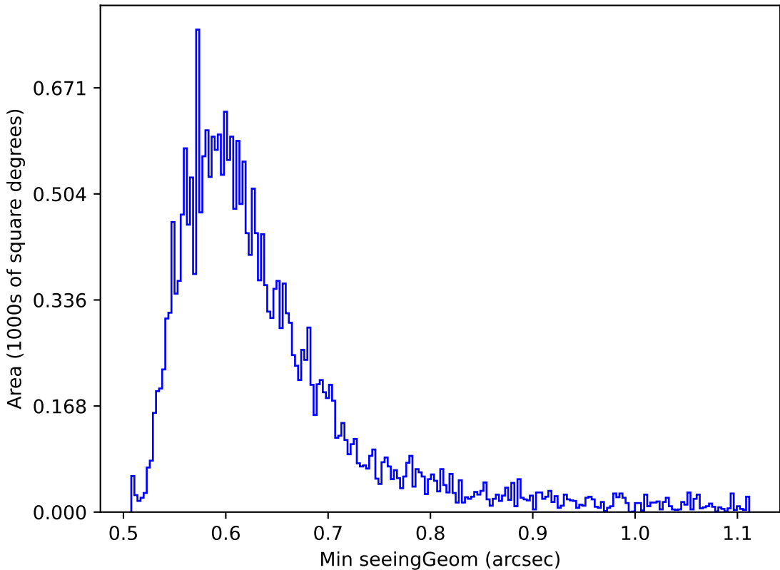
roll_pause_mjdp120_v3.4_10yrs Yr 1 i band: Min seeingGeom
