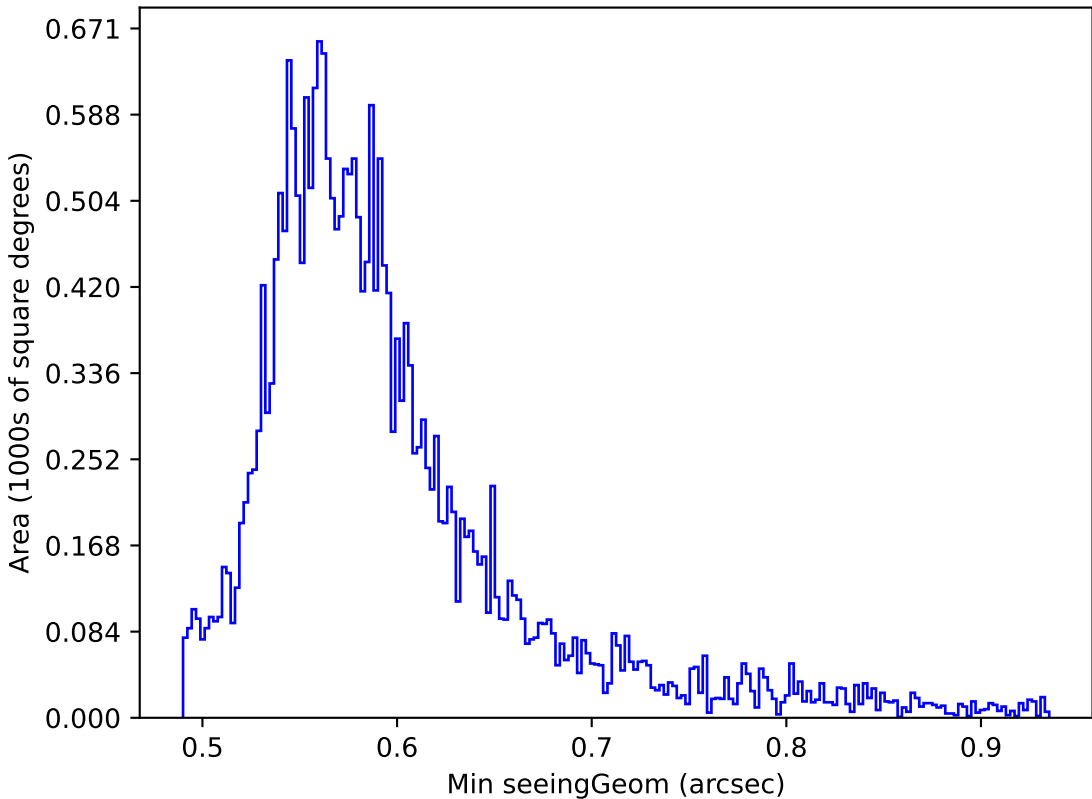
roll_pause_mjdp120_v3.4_10yrs Yr 1 all bands: Min seeingGeom
