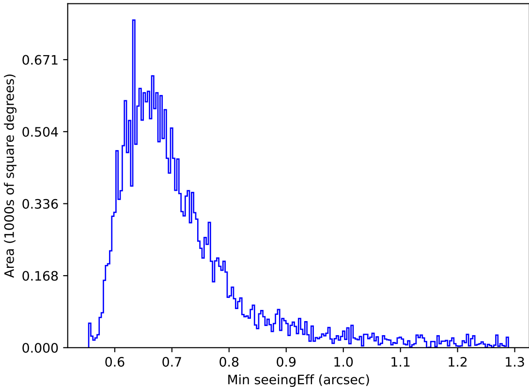
roll_pause_mjdp120_v3.4_10yrs Yr 1 i band: Min seeingEff
