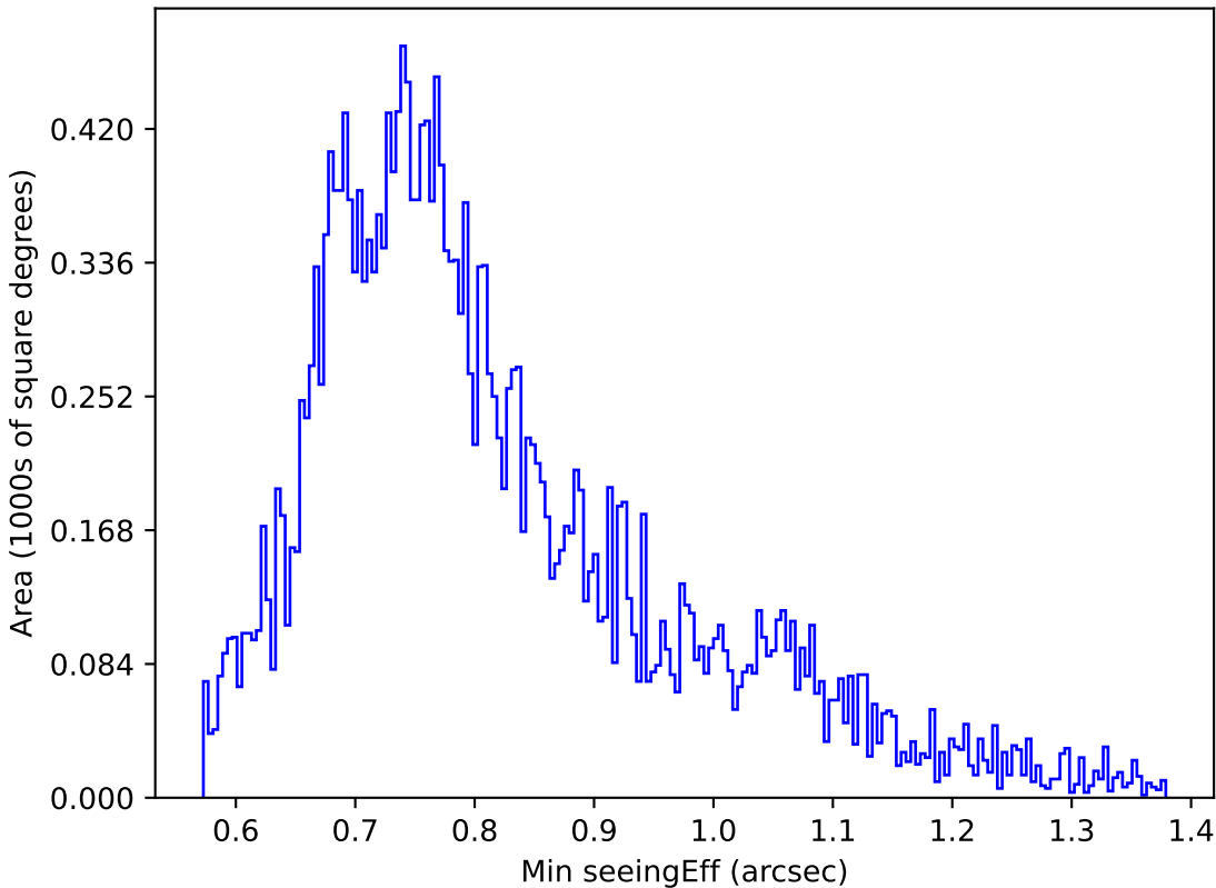
roll_pause_mjdp120_v3.4_10yrs Yr 1 g band: Min seeingEff
