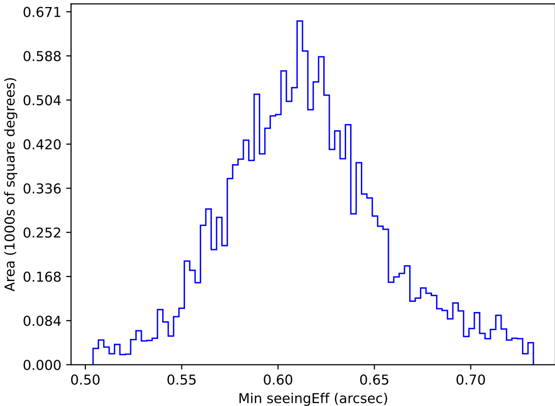
roll_pause_mjdp120_v3.4_10yrs WFD z band: Min seeingEff
