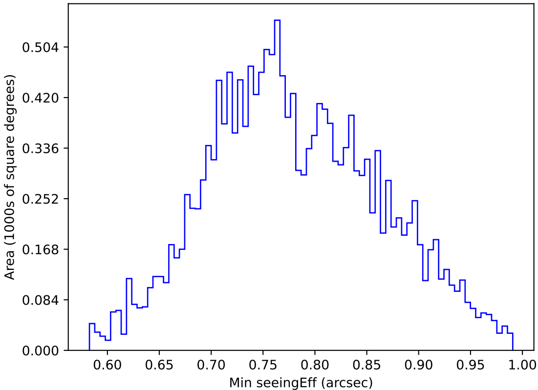
roll_pause_mjdp120_v3.4_10yrs WFD u band: Min seeingEff
