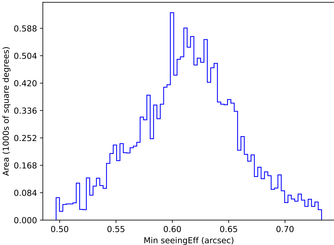
roll_pause_mjdp120_v3.4_10yrs WFD r band: Min seeingEff
