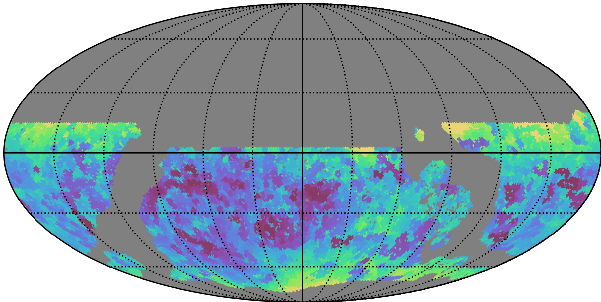
roll_pause_mjdp120_v3.4_10yrs WFD all bands: Min seeingEff
