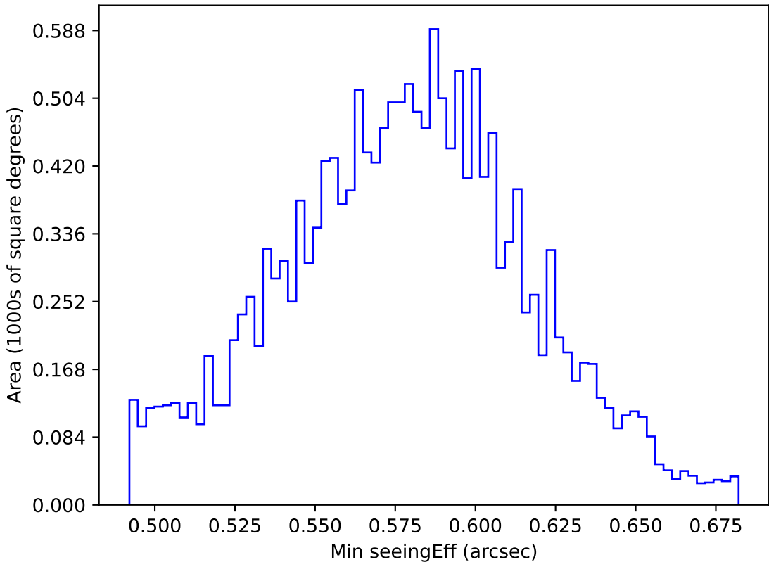
roll_pause_mjdp120_v3.4_10yrs WFD all bands: Min seeingEff
