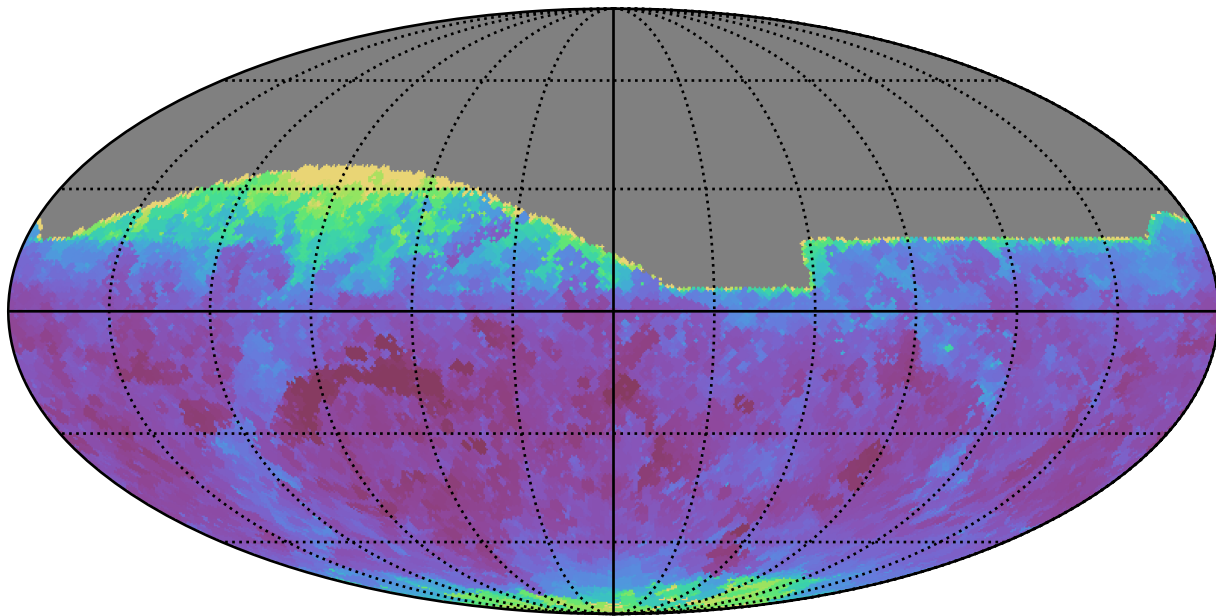
roll_pause_mjdp120_v3.4_10yrs All sky z band: Min seeingEff
