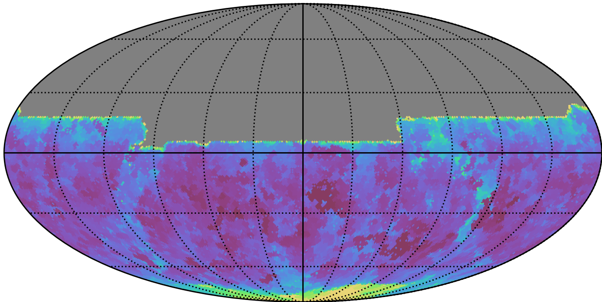
roll_pause_mjdp120_v3.4_10yrs All sky y band: Min seeingEff
