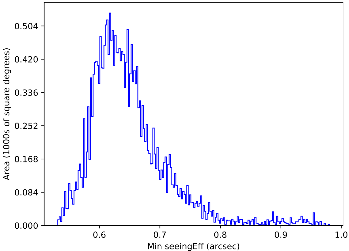
roll_pause_mjdp120_v3.4_10yrs All sky y band: Min seeingEff
