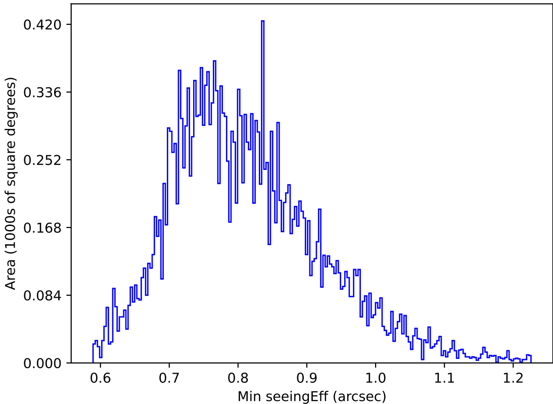
roll_pause_mjdp120_v3.4_10yrs All sky u band: Min seeingEff
