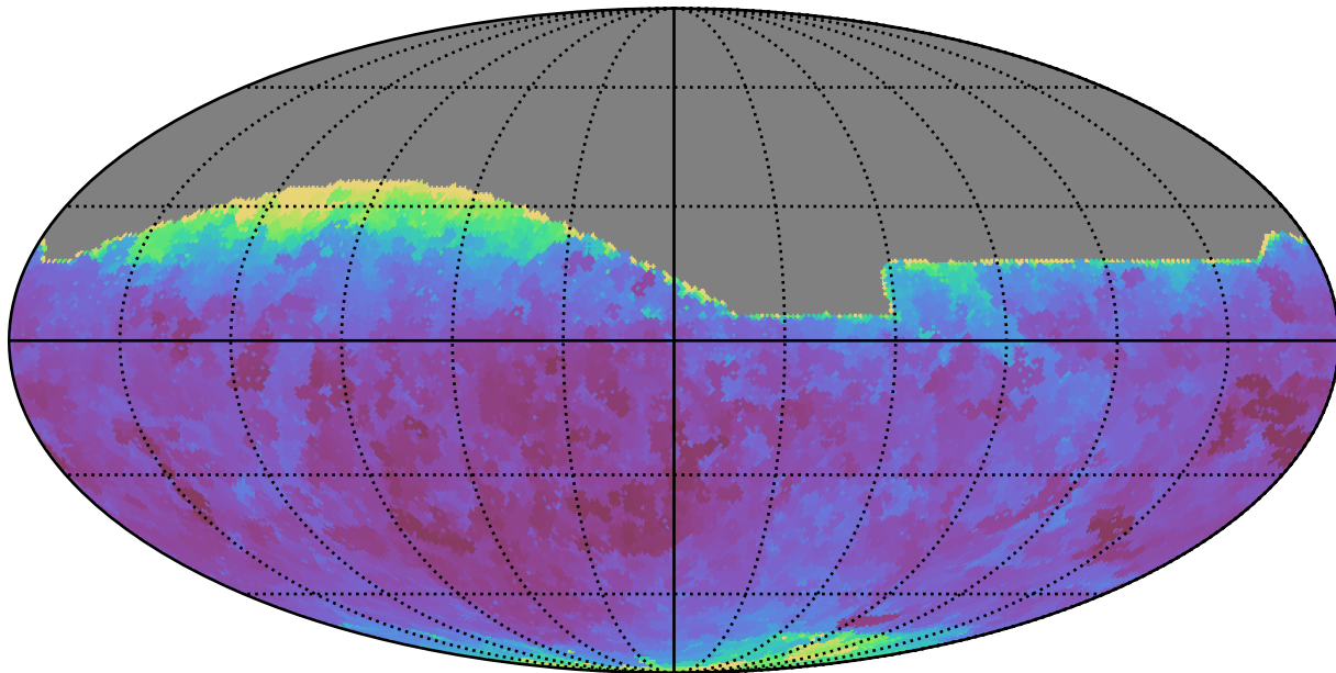
roll_pause_mjdp120_v3.4_10yrs All sky r band: Min seeingEff
