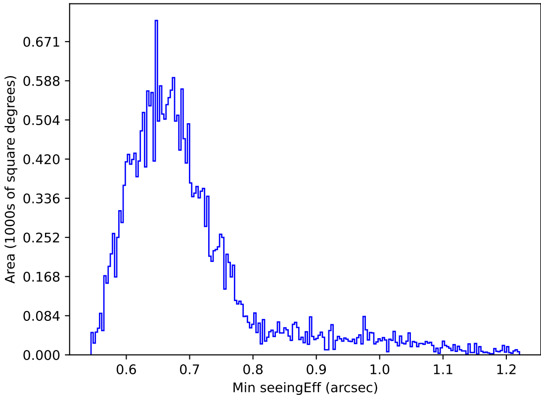
roll_pause_mjdp120_v3.4_10yrs All sky g band: Min seeingEff
