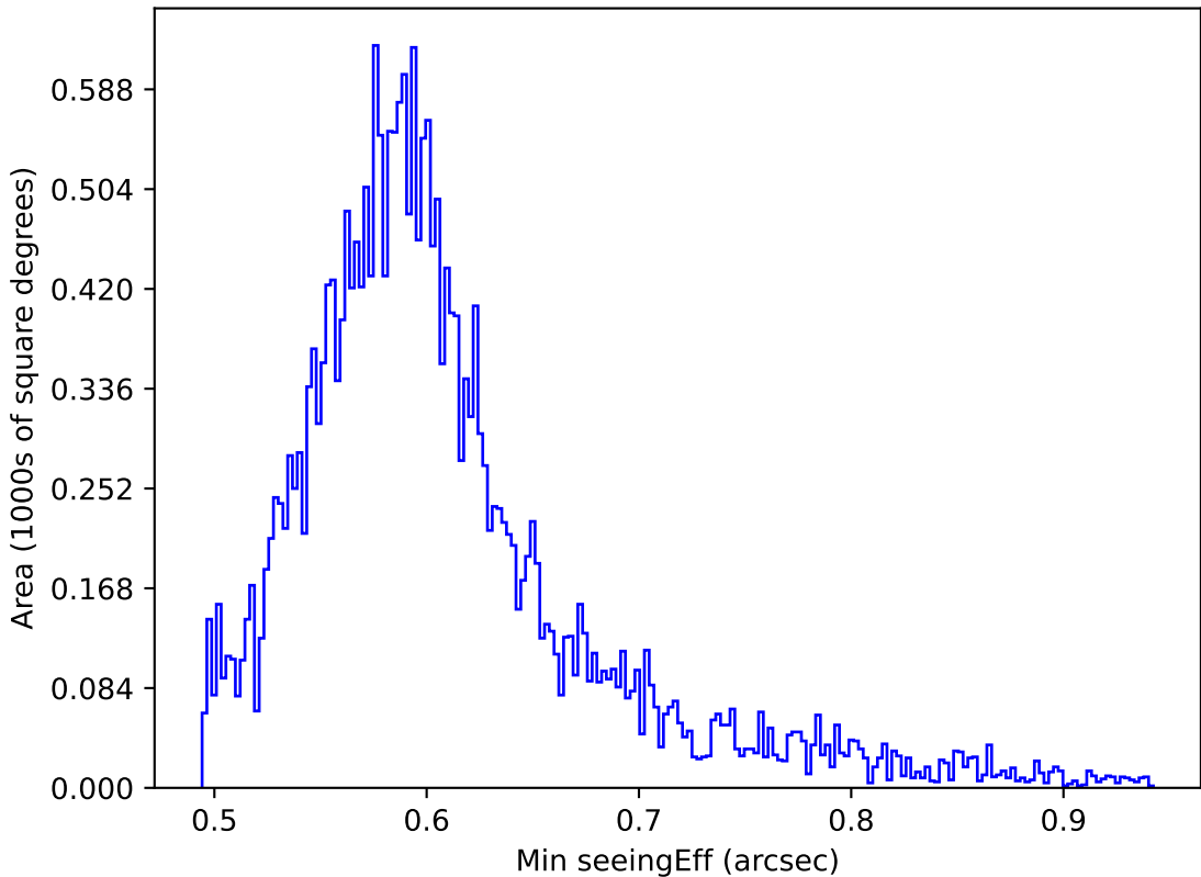
roll_pause_mjdp120_v3.4_10yrs All sky all bands: Min seeingEff
