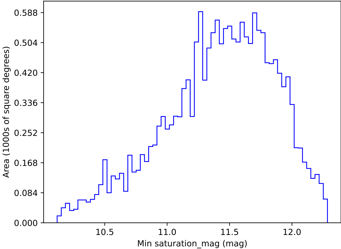
roll_pause_mjdp120_v3.4_10yrs WFD u band: Min saturation_mag
