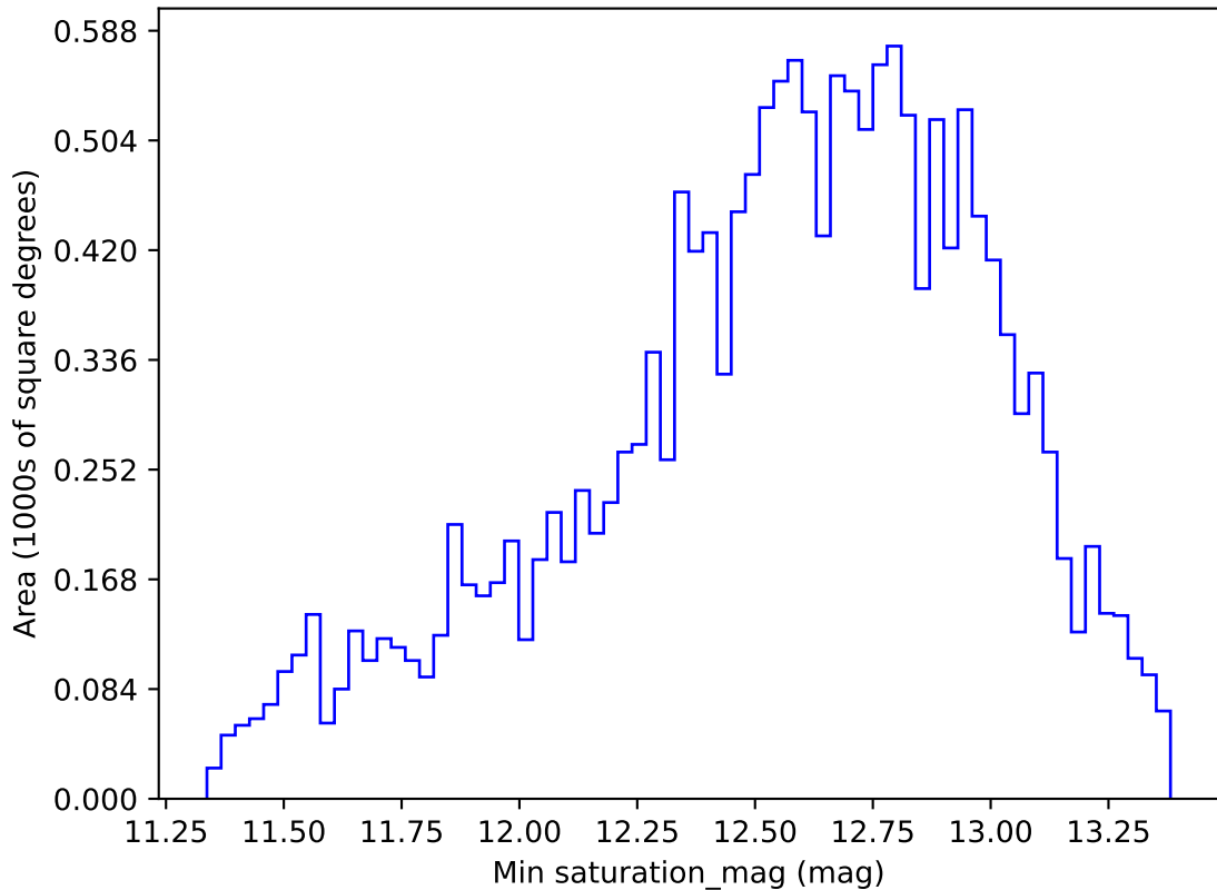
roll_pause_mjdp120_v3.4_10yrs WFD r band: Min saturation_mag
