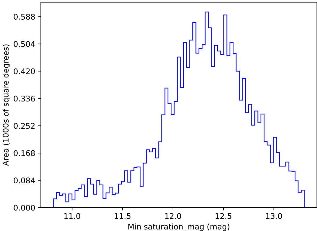
roll_pause_mjdp120_v3.4_10yrs WFD i band: Min saturation_mag
