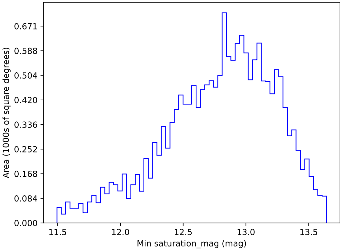
roll_pause_mjdp120_v3.4_10yrs WFD g band: Min saturation_mag
