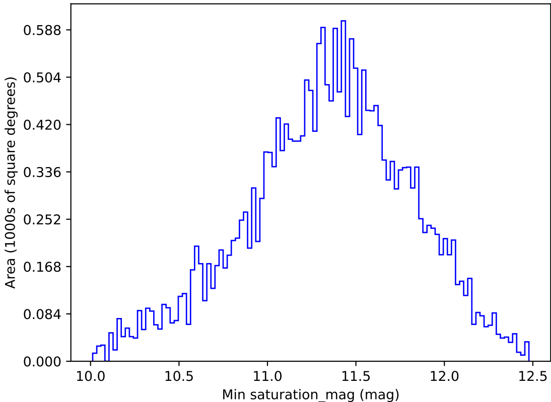
roll_pause_mjdp120_v3.4_10yrs All sky y band: Min saturation_mag
