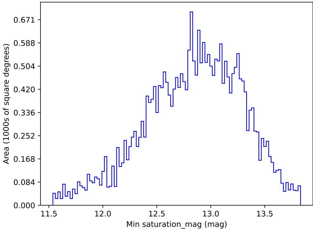
roll_pause_mjdp120_v3.4_10yrs All sky g band: Min saturation_mag
