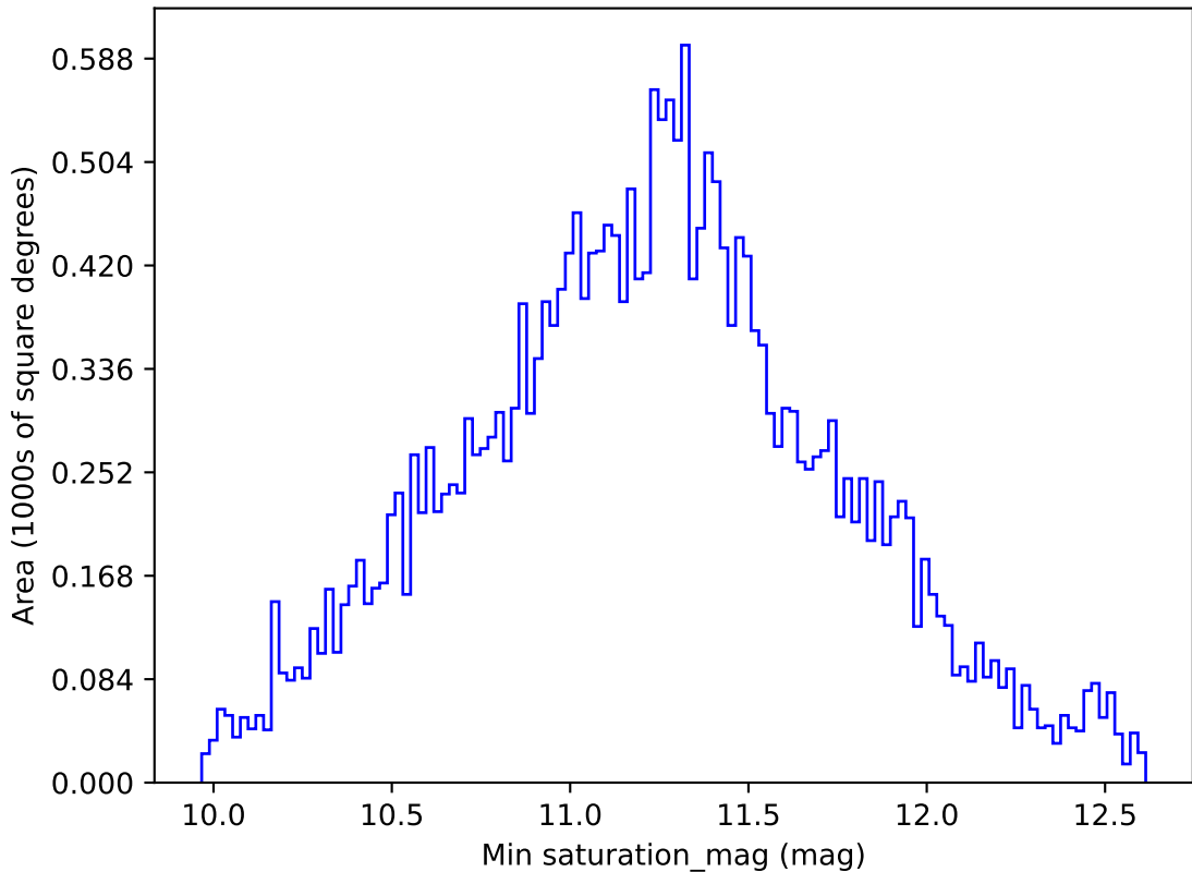
roll_pause_mjdp120_v3.4_10yrs All sky all bands: Min saturation_mag
