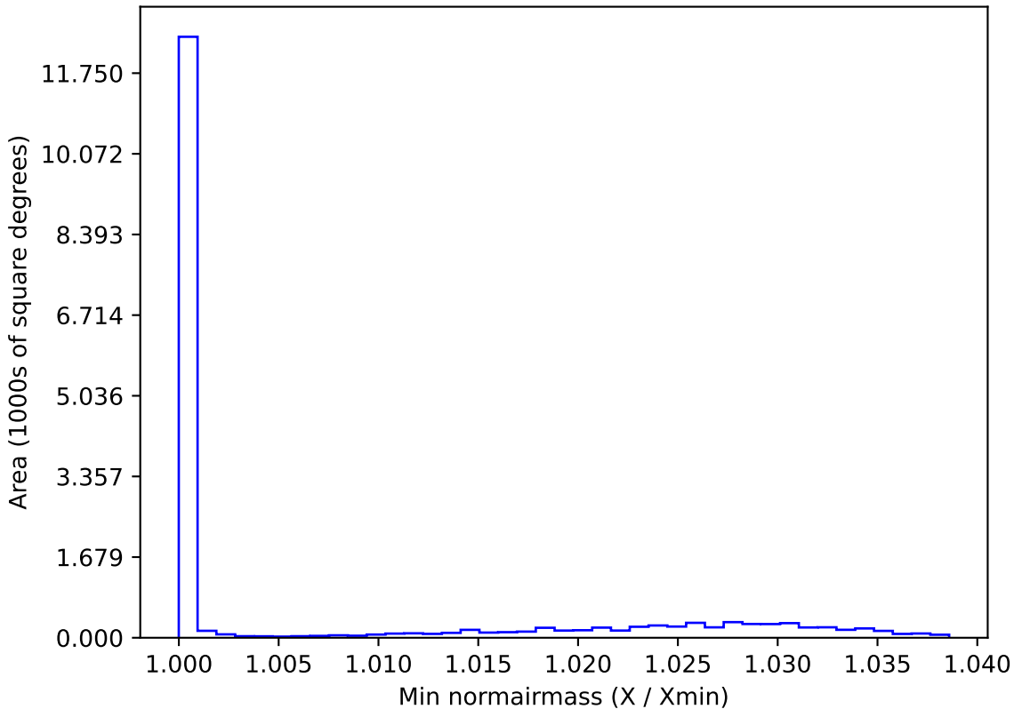
roll_pause_mjdp120_v3.4_10yrs WFD y band: Min normairmass
