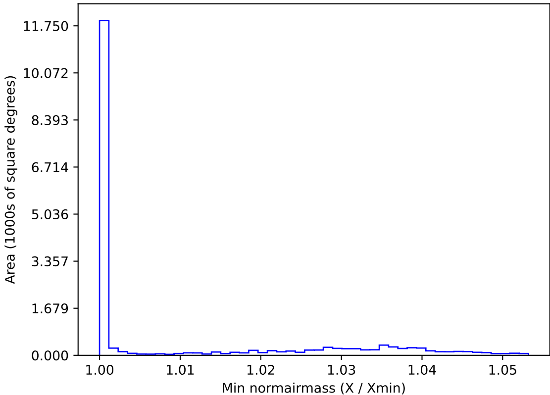
roll_pause_mjdp120_v3.4_10yrs WFD u band: Min normairmass
