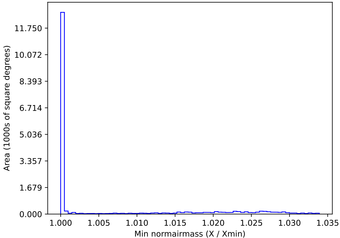
roll_pause_mjdp120_v3.4_10yrs WFD r band: Min normairmass
