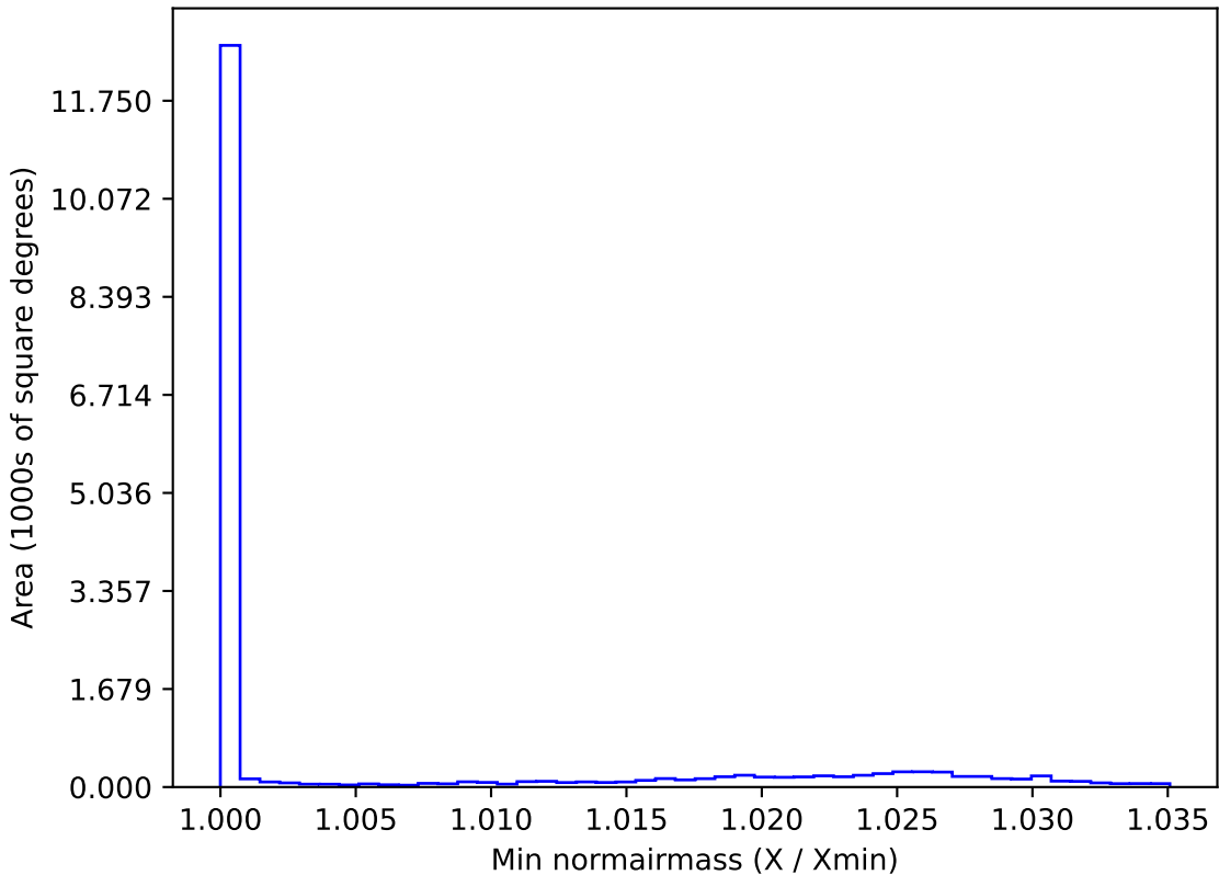
roll_pause_mjdp120_v3.4_10yrs WFD i band: Min normairmass
