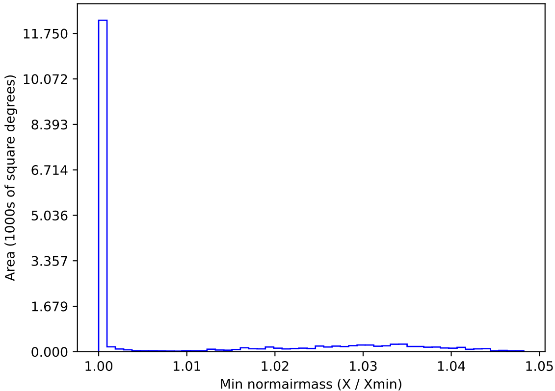
roll_pause_mjdp120_v3.4_10yrs WFD g band: Min normairmass
