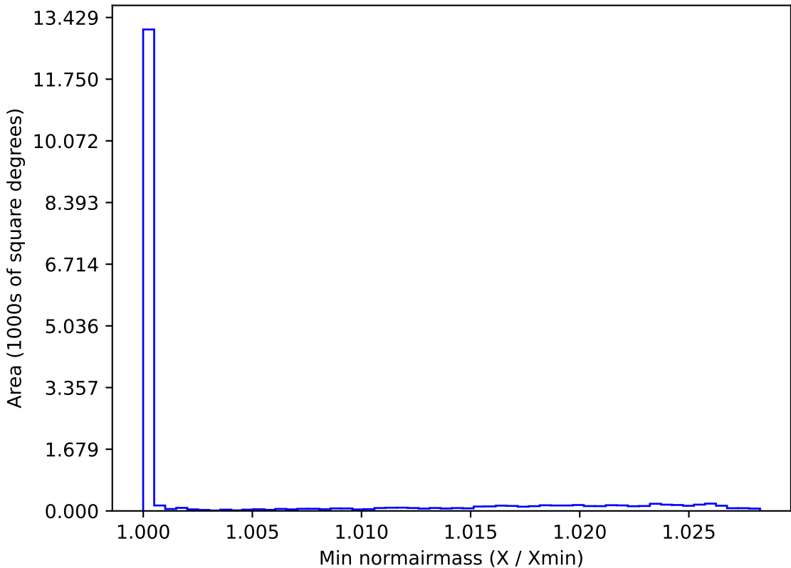
roll_pause_mjdp120_v3.4_10yrs WFD all bands: Min normairmass
