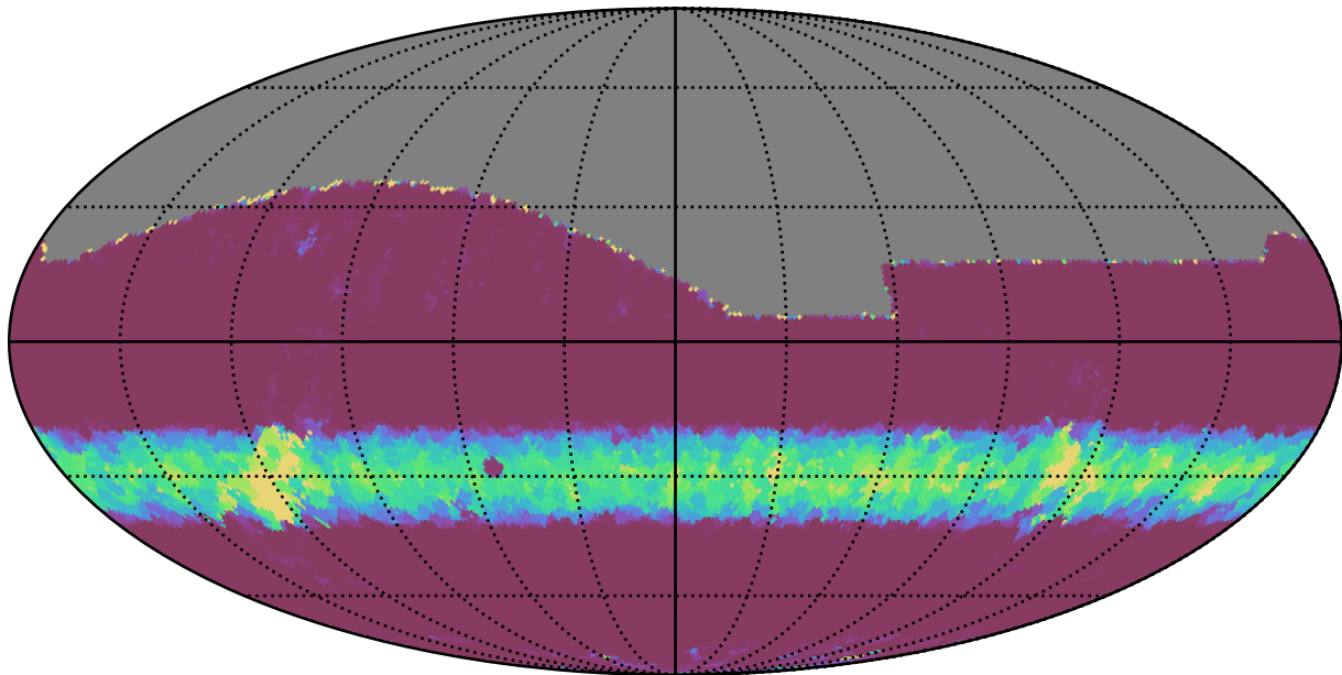
roll_pause_mjdp120_v3.4_10yrs All sky z band: Min normairmass
