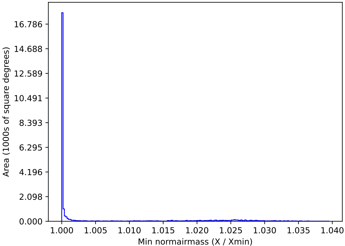
roll_pause_mjdp120_v3.4_10yrs All sky z band: Min normairmass
