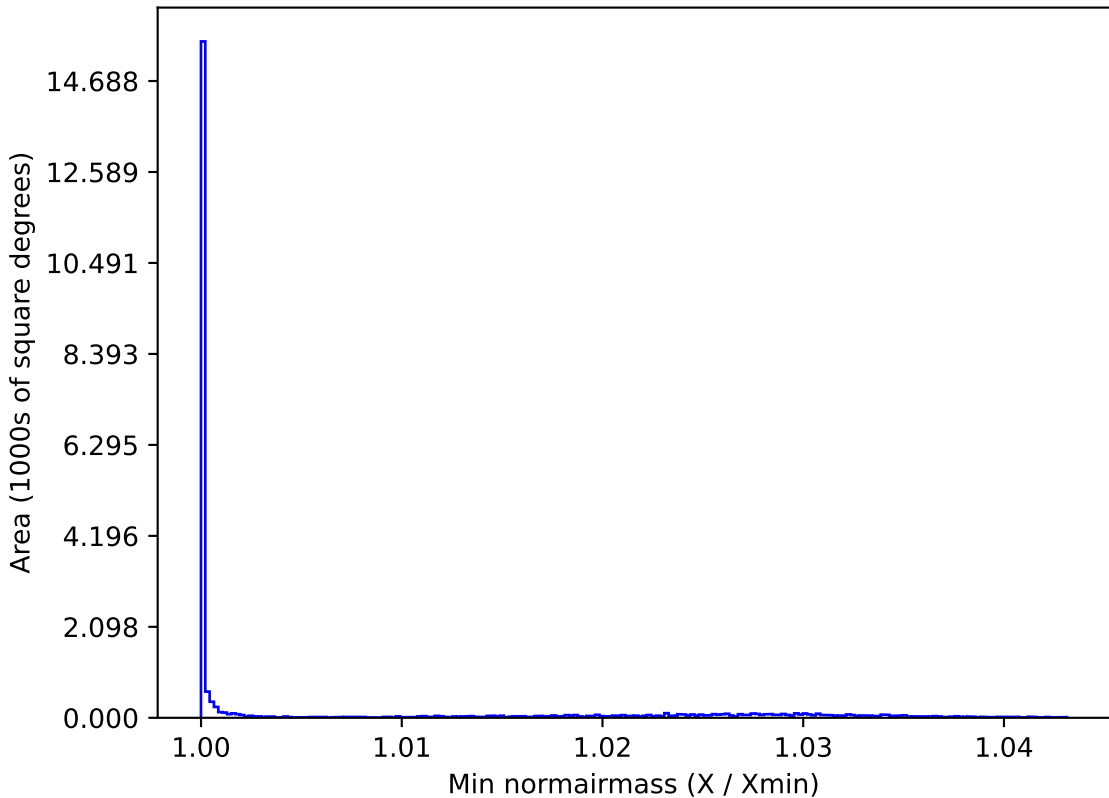
roll_pause_mjdp120_v3.4_10yrs All sky y band: Min normairmass
