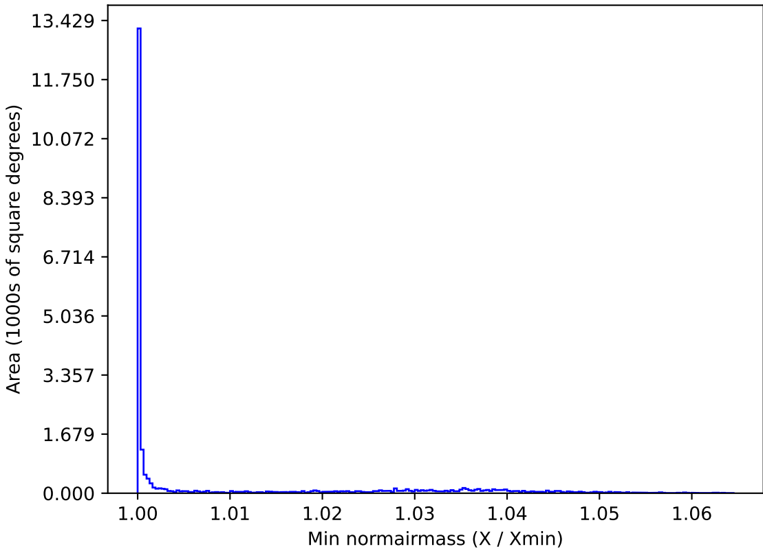
roll_pause_mjdp120_v3.4_10yrs All sky u band: Min normairmass
