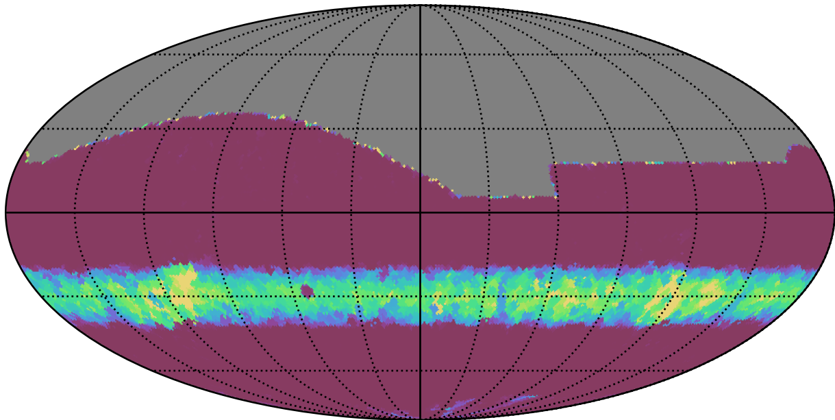
roll_pause_mjdp120_v3.4_10yrs All sky i band: Min normairmass
