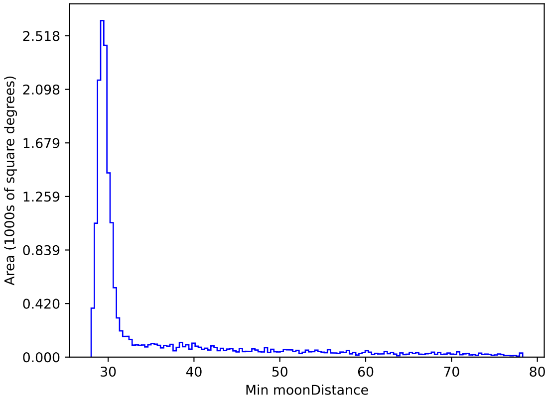
roll_pause_mjdp120_v3.4_10yrs WFD y band: Min moonDistance
