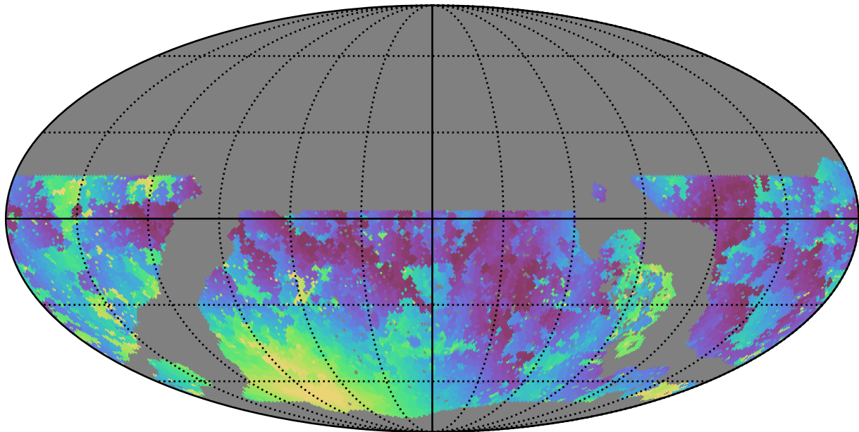
roll_pause_mjdp120_v3.4_10yrs WFD u band: Min moonDistance
