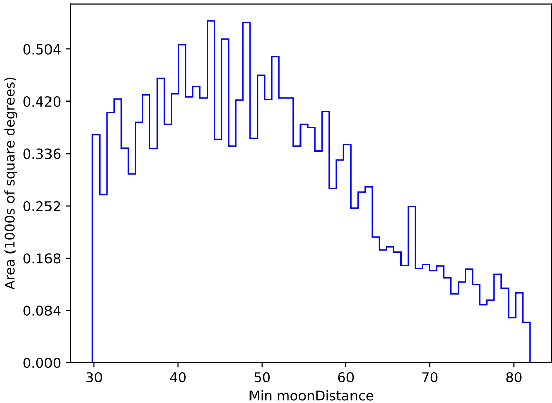
roll_pause_mjdp120_v3.4_10yrs WFD u band: Min moonDistance
