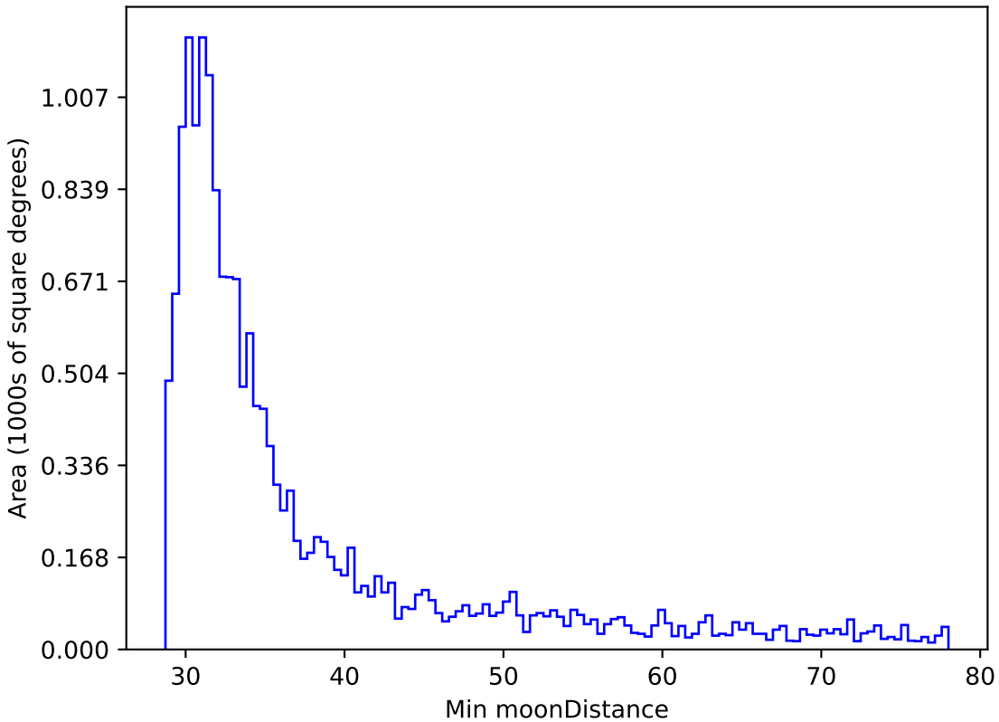
roll_pause_mjdp120_v3.4_10yrs WFD r band: Min moonDistance
