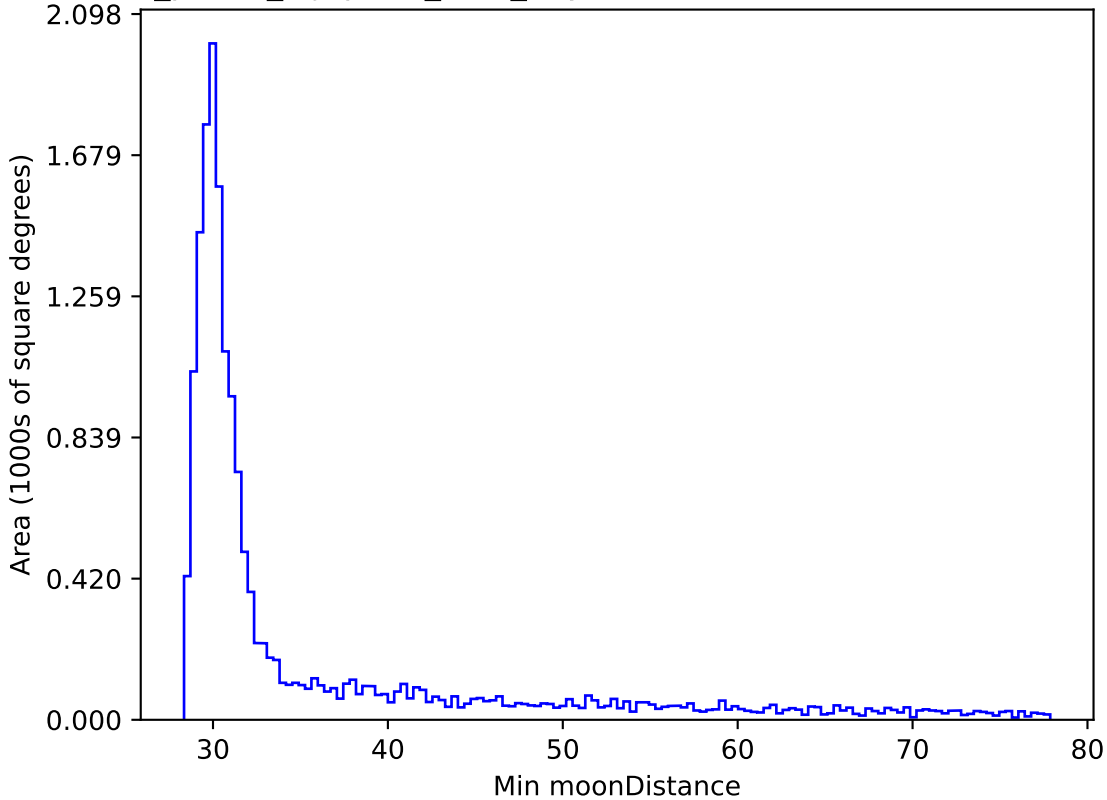
roll_pause_mjdp120_v3.4_10yrs WFD i band: Min moonDistance
