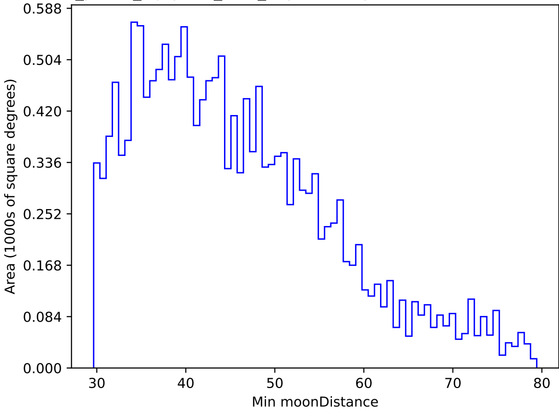
roll_pause_mjdp120_v3.4_10yrs WFD g band: Min moonDistance
