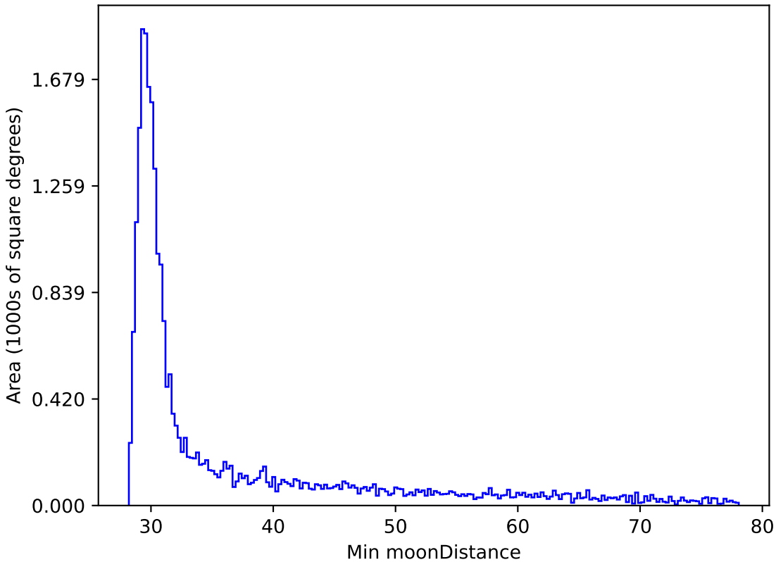
roll_pause_mjdp120_v3.4_10yrs All sky z band: Min moonDistance
