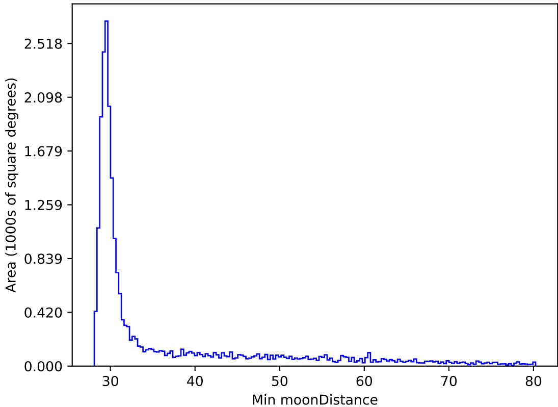
roll_pause_mjdp120_v3.4_10yrs All sky y band: Min moonDistance
