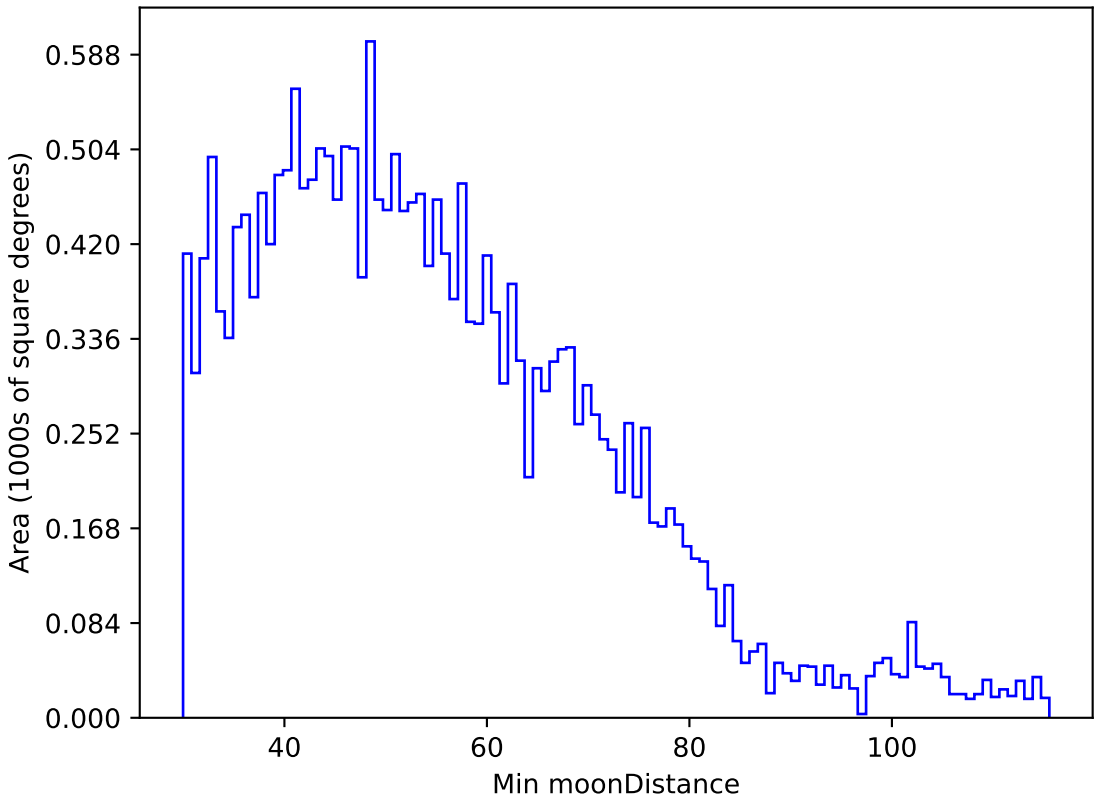
roll_pause_mjdp120_v3.4_10yrs All sky u band: Min moonDistance
