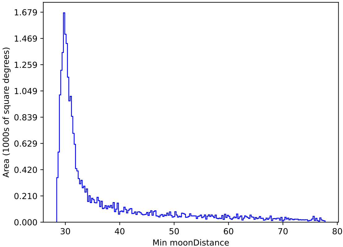
roll_pause_mjdp120_v3.4_10yrs All sky i band: Min moonDistance
